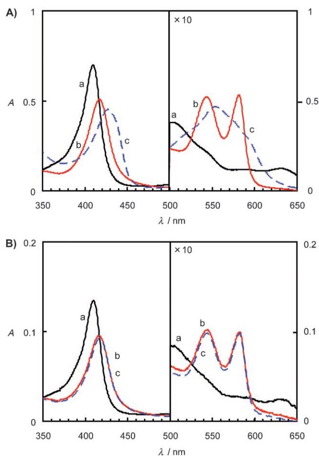
Figure 3. A) Electronic absorption spectra a) of free Mb solution ( 60 \mu\text{g mL}^{-1} ; black solid line), b) after reduction and further introduction of O_2 gas in the absence of trypsin (red solid line), and c) after incubation with trypsin ( 37^\circ\text{C} , 4 h; blue dashed line). B) Electronic absorption spectra a) of the solution of Mb-loaded PICsomes (black solid line), b) after reduction and further introduction of O_2 gas in the absence of trypsin (red solid line), and c) after incubation with trypsin ( 37^\circ\text{C} , 4 h; blue dashed line).
